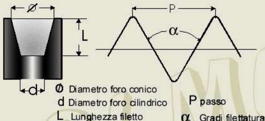
NPT Gas conica americana 1:16
